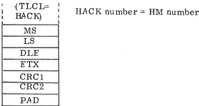
fig. 6.2.3 Hello Ack
