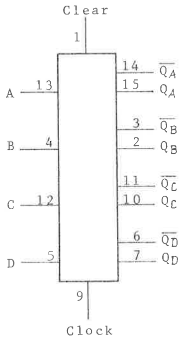
74175 Quadruple D-type flip-flop with clear
