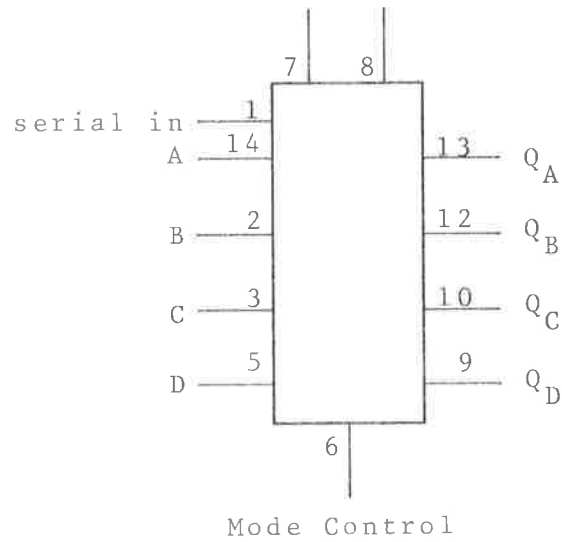
74L95 4-bit parallel-access shift register
