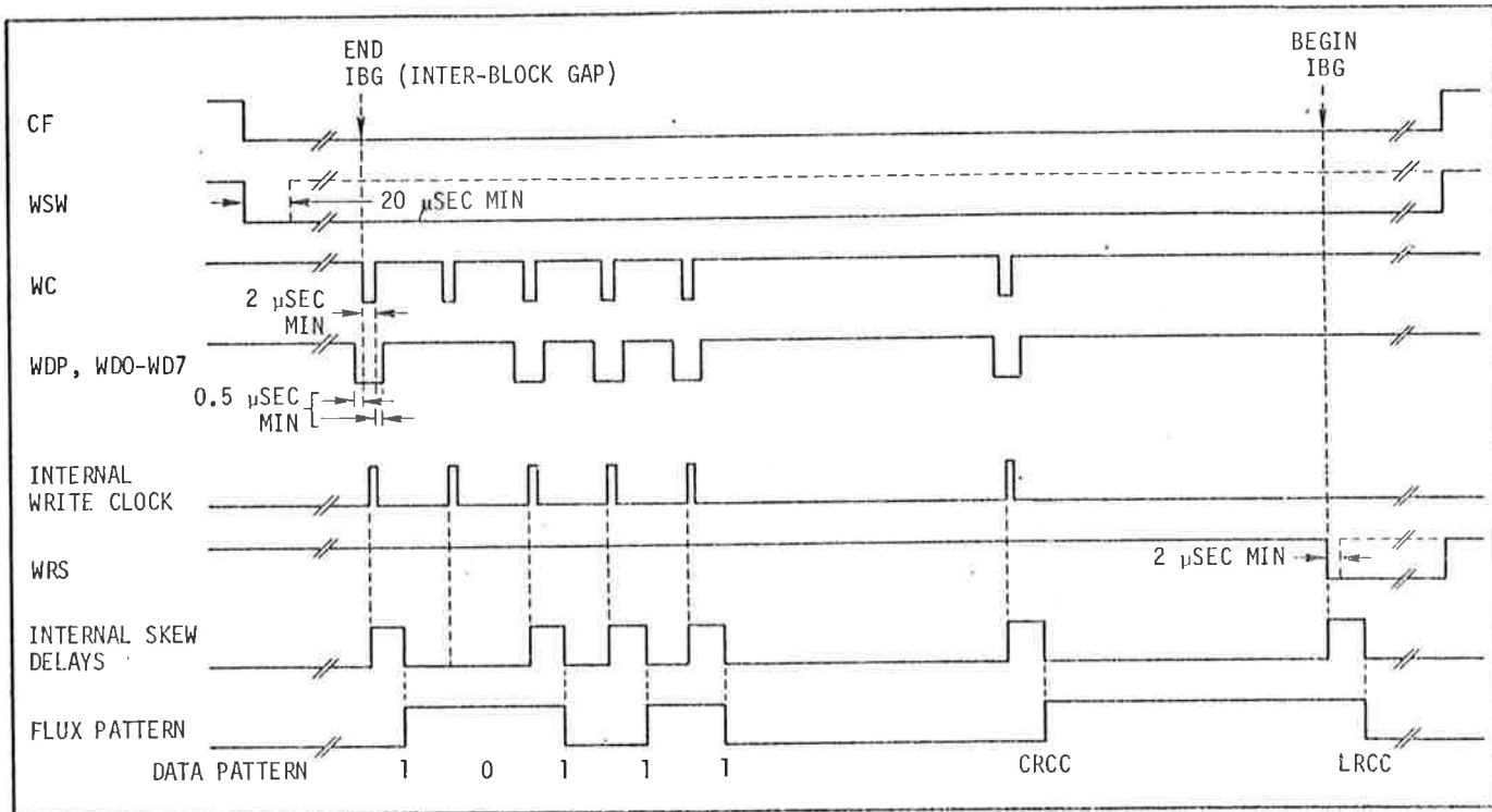
Figure 2. Write Waveforms
