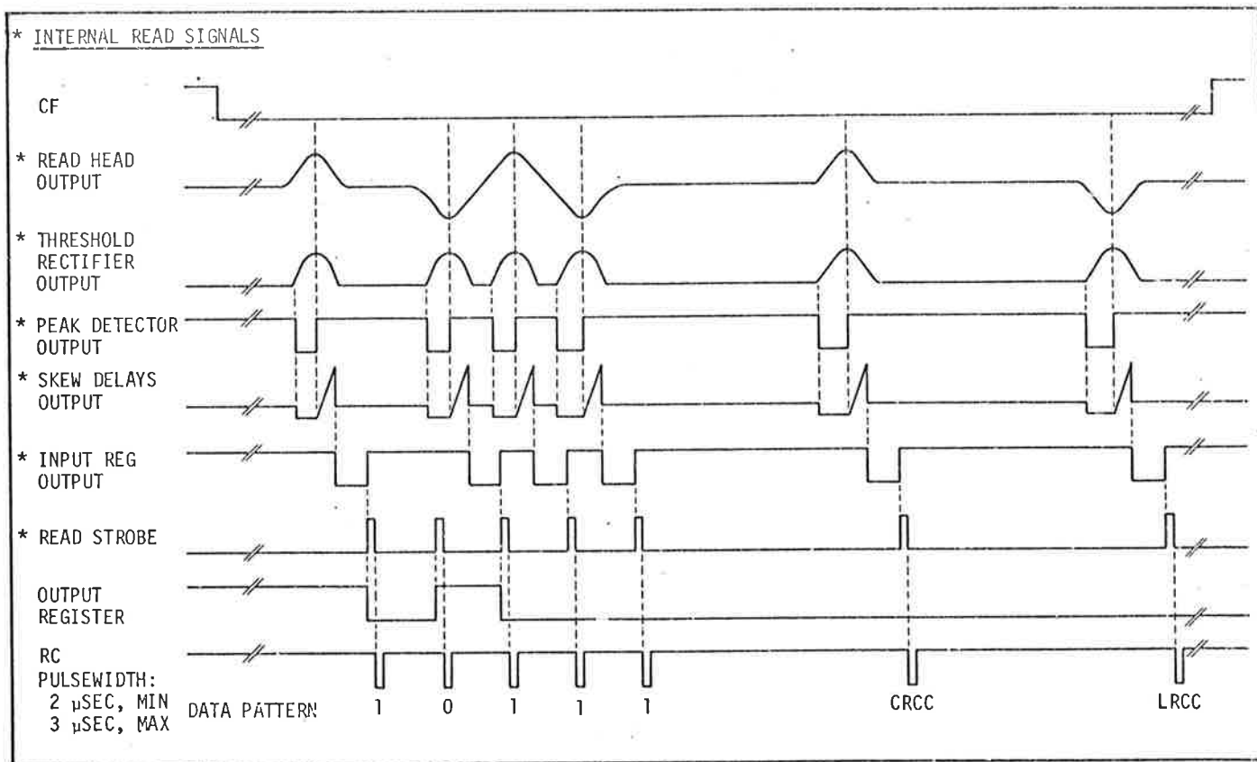
Figure 3. Read Waveforms
