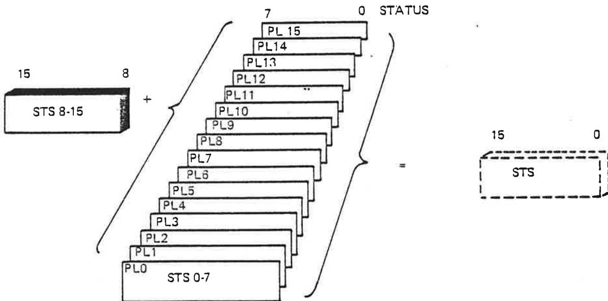
Figure 2.3: Register File
