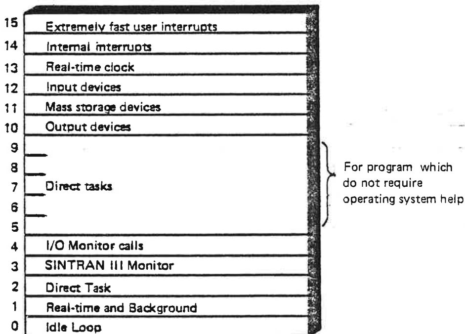
Figure 2.5: Level Assignments
