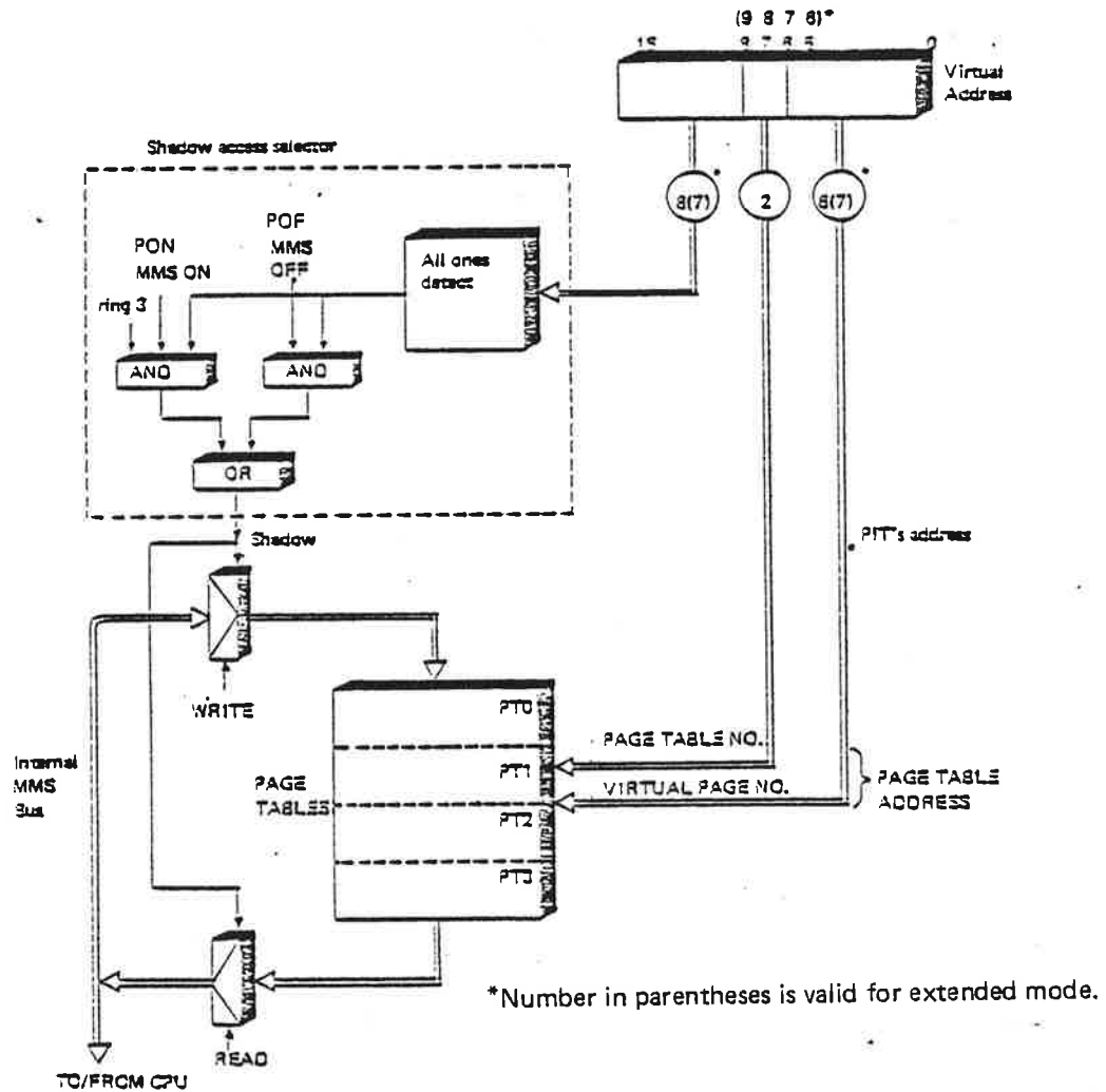
Figure 2.12: Shadow Memory Addressing.
